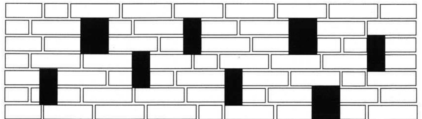
透かし乱積 Honeycomb brick work
